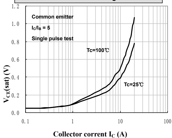
Saturation Voltage
