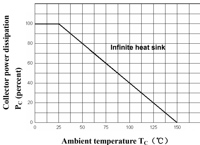
Power Derating
