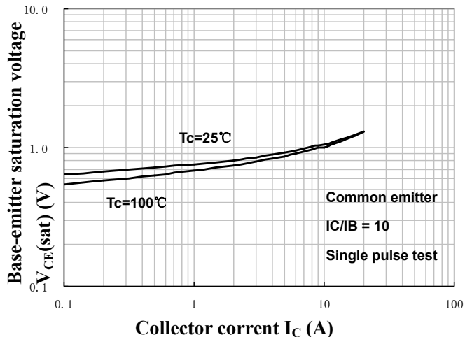
Base-Emitter Voltage
